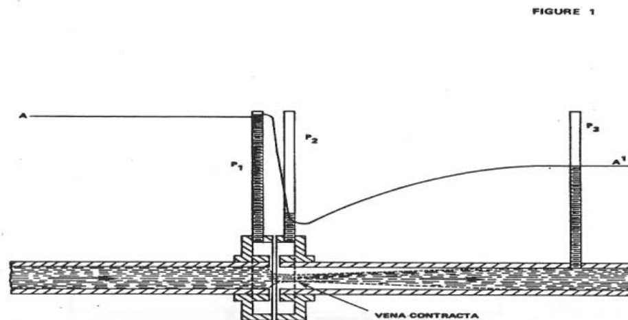
Figure 2. Vena Contracta
