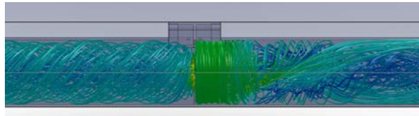
Figure 14: Visualization of velocity trajectories as flow with heavy swirl passes through an orifice meter.
