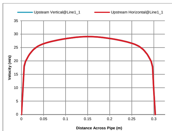
Figure 8: Fully developed flow profiles in a turbulent flow, Re \sim 30,000,000 .
