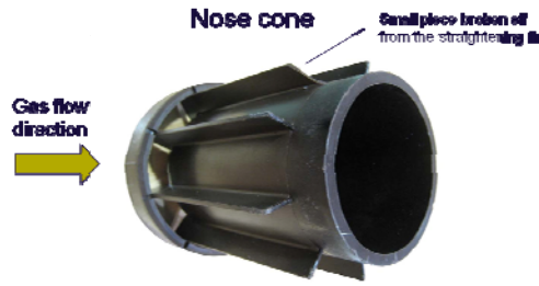
Figure 7. Damaged Nose Cone
