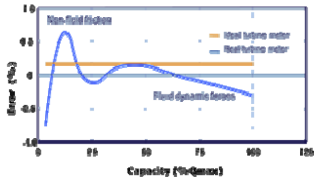
Figure 2. Effect of Fluid and Non-fluid Retarding Torques on Gas Turbine Meter Performance
