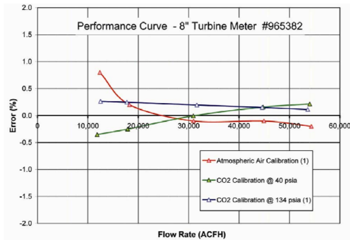
Figure 10. Line Pressure Effect on Turbine Meter Flow Measurement Error
