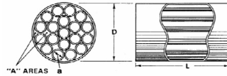
Conventional tube bundle straightening vanes
