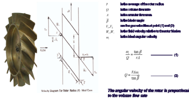
Figure 1. Angular Velocity of a Turbine Meter Rotor
