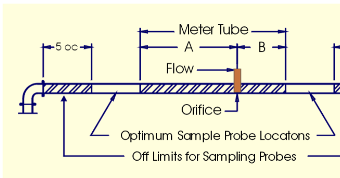
Figure 1; Optimum Sample Probe Locations
