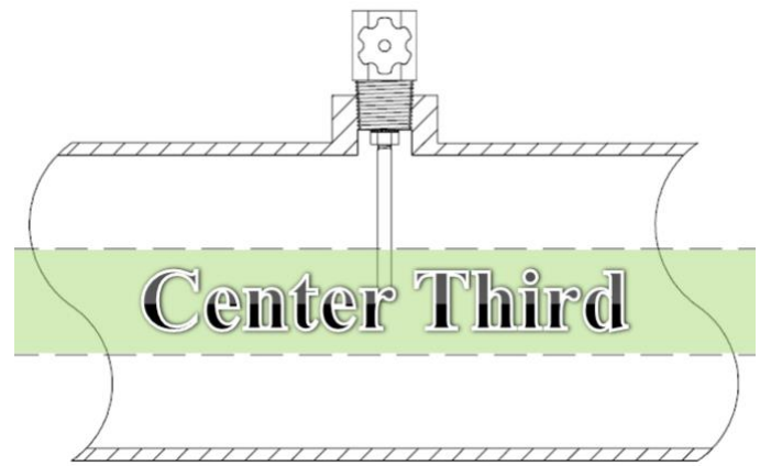
Figure 2; Sample Probe Insertion Depth
